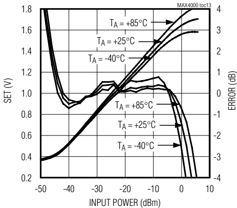
MAX4000 SET AND LOG CONFORMANCE vs. INPUT POWER AT 1.9GHz
