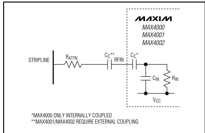
Figure 3c. Series Attenuation Network
