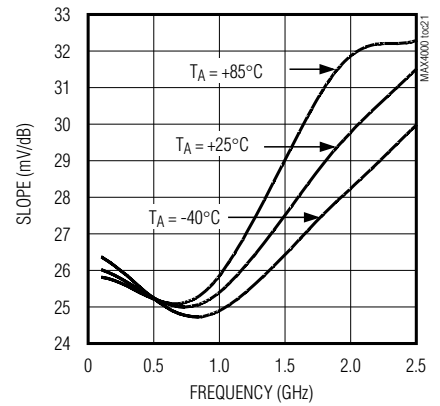
MAX4002 SLOPE vs. FREQUENCY
