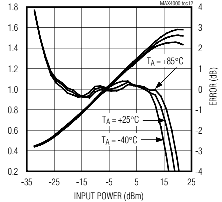
MAX4002 SET AND LOG CONFORMANCE vs. INPUT POWER AT 0.9GHz
