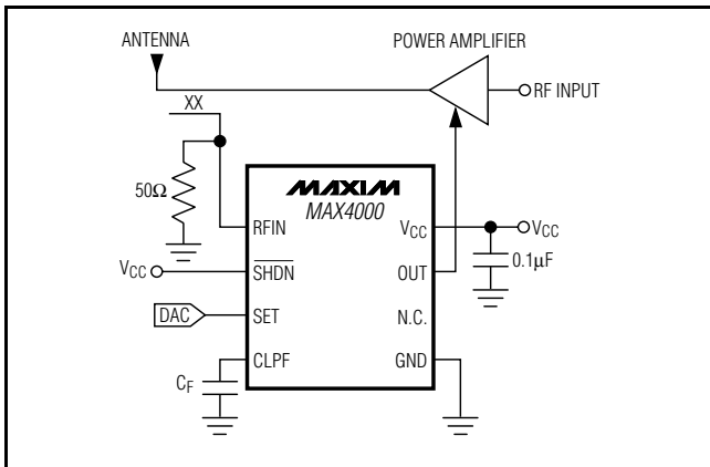
Figure 2. Controller Mode Application Circuit Block
