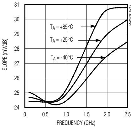
MAX4000 SLOPE vs. FREQUENCY
