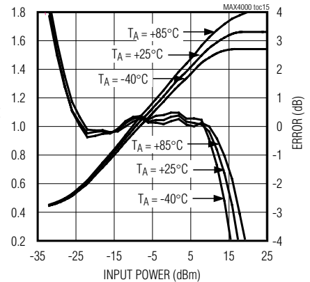
MAX4002 SET AND LOG CONFORMANCE vs. INPUT POWER AT 1.9GHz
