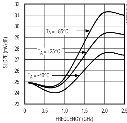
MAX4001 SLOPE vs. FREQUENCY
