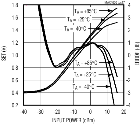
MAX4001 SET AND LOG CONFORMANCE vs. INPUT POWER AT 2.5GHz
