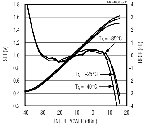
MAX4001 SET AND LOG CONFORMANCE vs. INPUT POWER AT 0.9GHz
