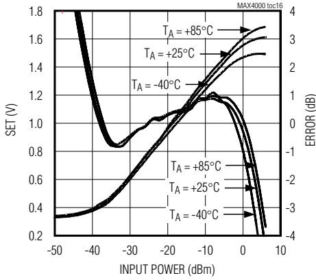
MAX4000 SET AND LOG CONFORMANCE vs. INPUT POWER AT 2.5GHz
