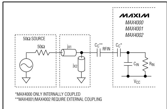
Figure 3b. Narrowband Reactive Matching
