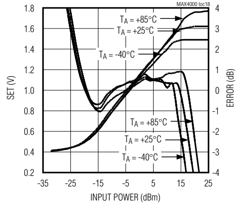
MAX4002 SET AND LOG CONFORMANCE vs. INPUT POWER AT 2.5GHz
