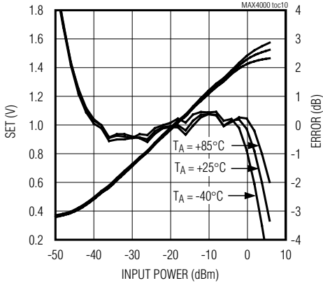
MAX4000 SET AND LOG CONFORMANCE vs. INPUT POWER AT 0.9GHz
