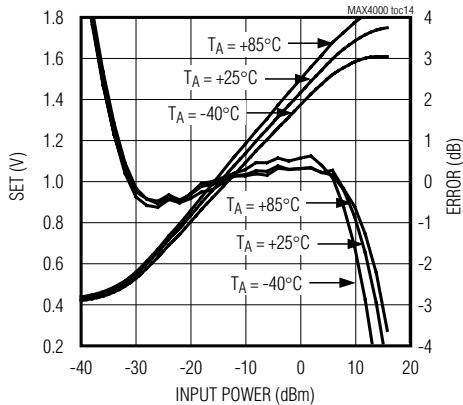
MAX4001 SET AND LOG CONFORMANCE vs. INPUT POWER AT 1.9GHz
