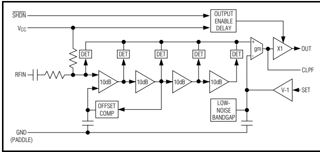
Figure 1. Functional Diagram
