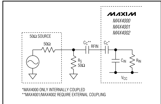
Figure 3a. Broadband Resistive Matching
